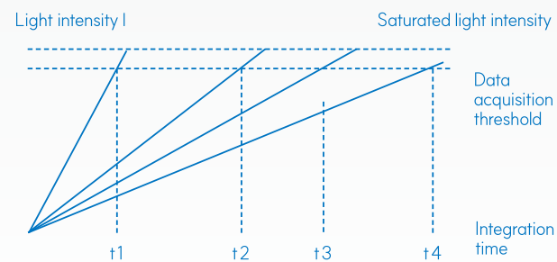
Schematic diagram for self-adaptive integration data acquisition system
